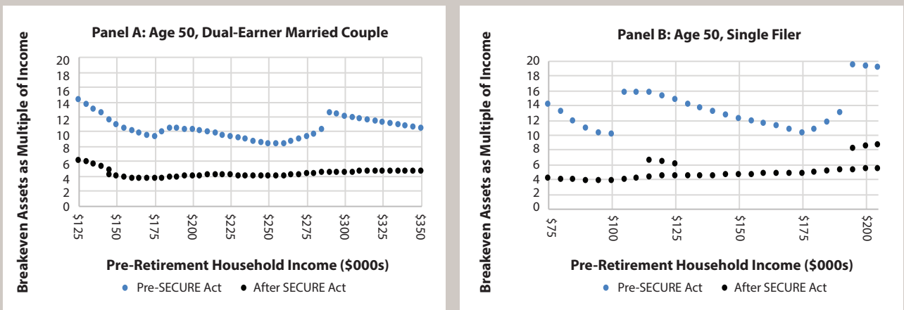
Figure 4: Breakeven Asset Levels Before and After the SECURE Act (Under Baseline Assumptions)
