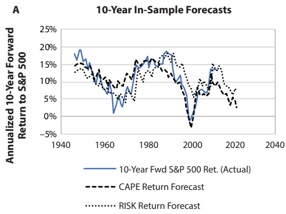
Figure 3: Forecast Comparison - CAPE vs RISK
